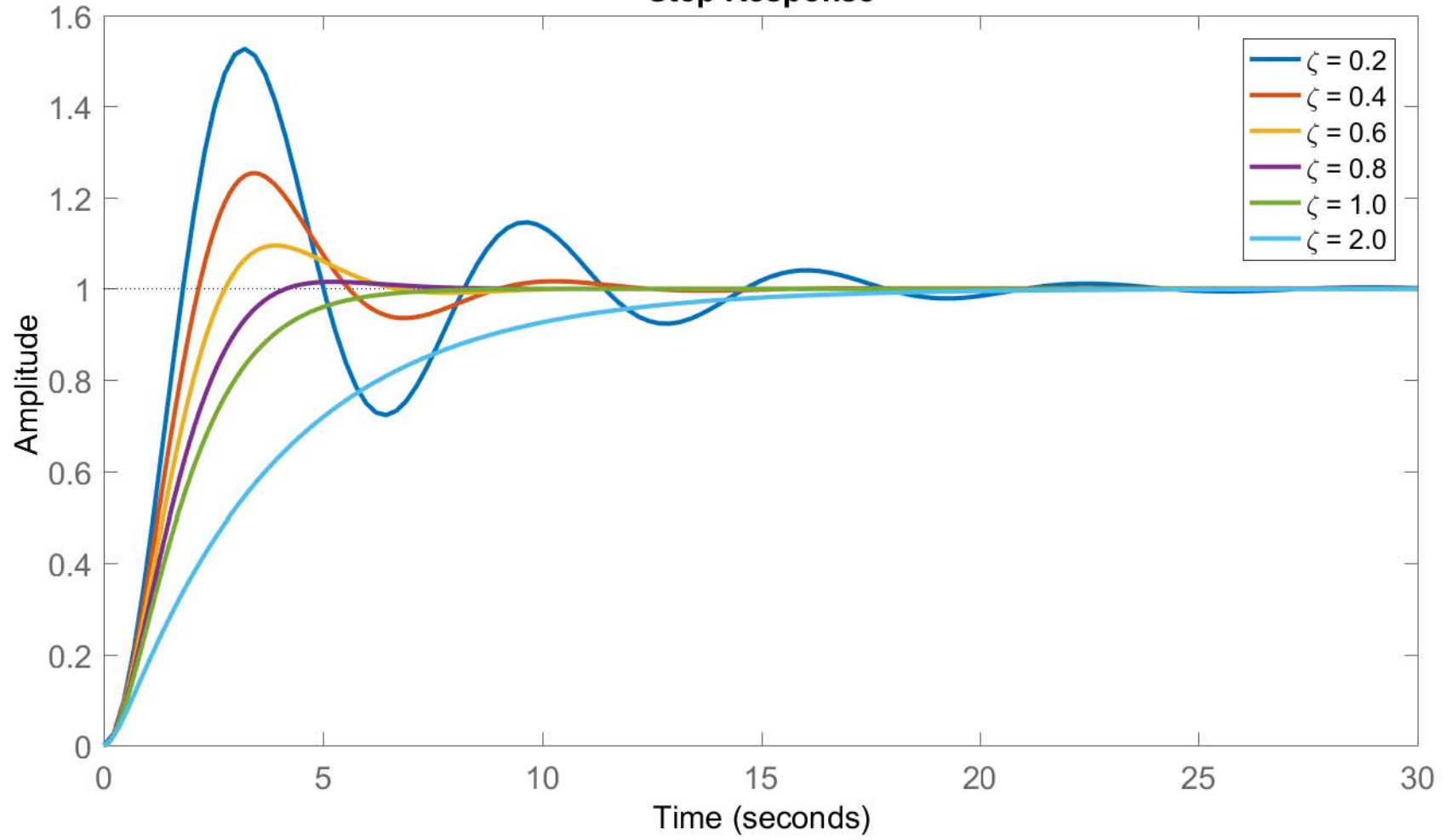
Step Response
